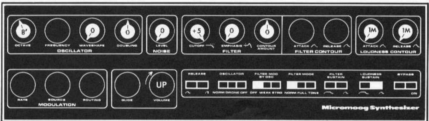
FIGURE 4-4 VCA BALANCE & TRILL TRIM SOUND CHART
