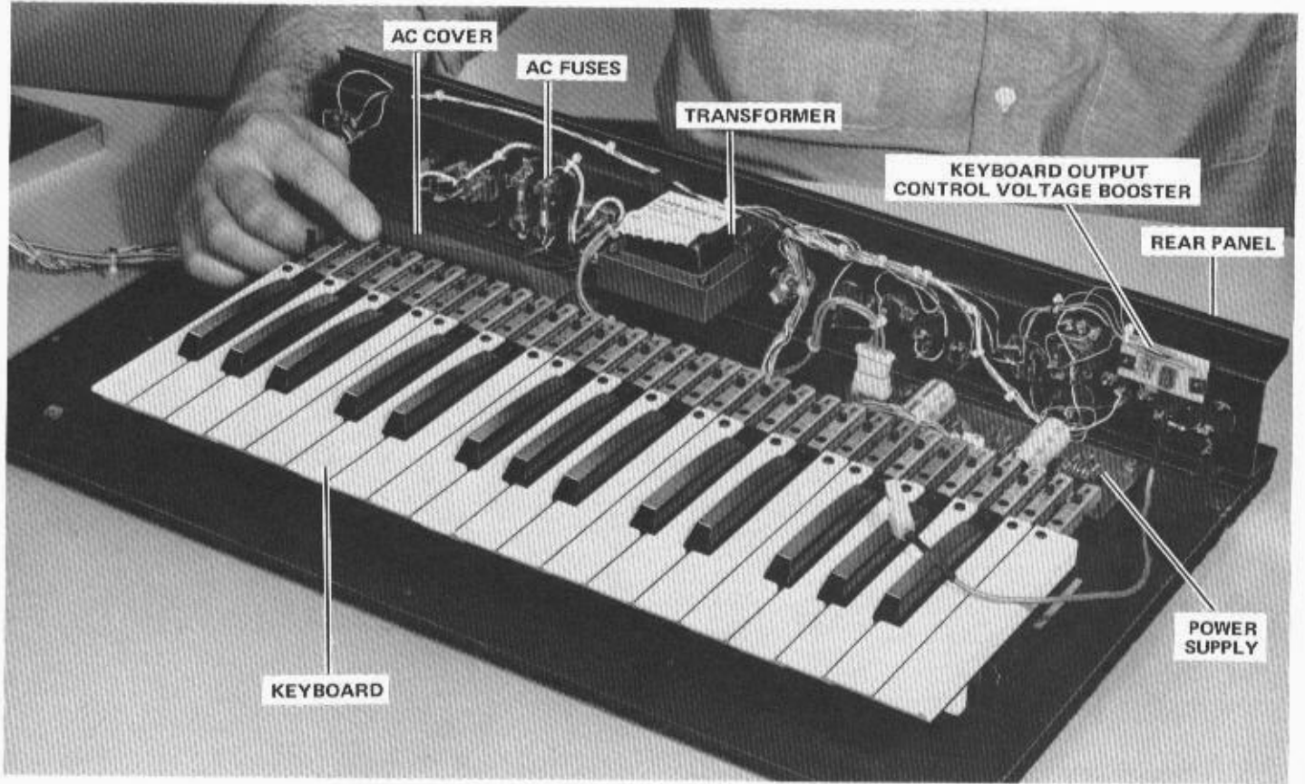
FIGURE 3-4 BASE ASSEMBLY
