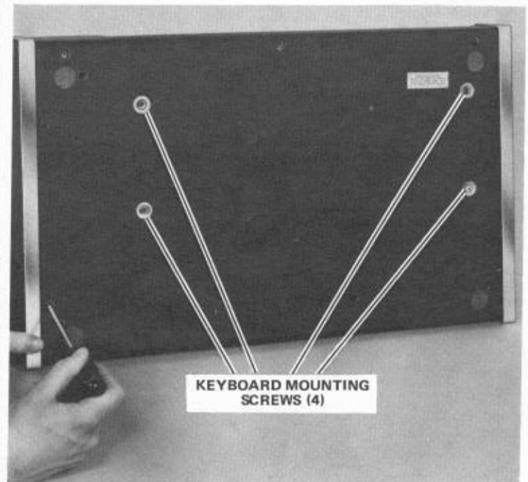
FIGURE 3-8 KEYBOARD MOUNTING
