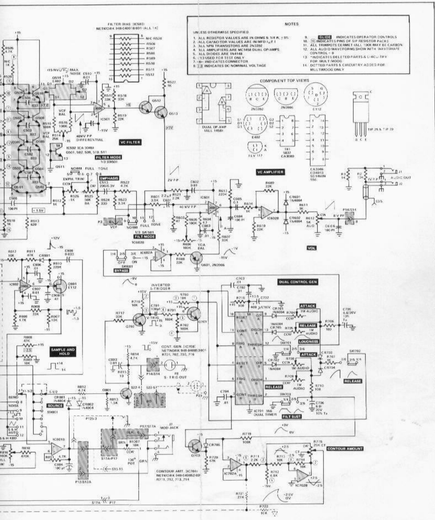
FIGURE 6-3 MICROMOG SCHEMATIC DIAGRAM
