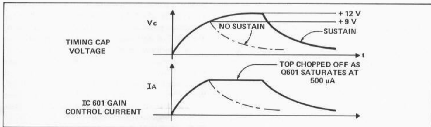
FIGURE 2-10 LOUDNESS LIMITING
