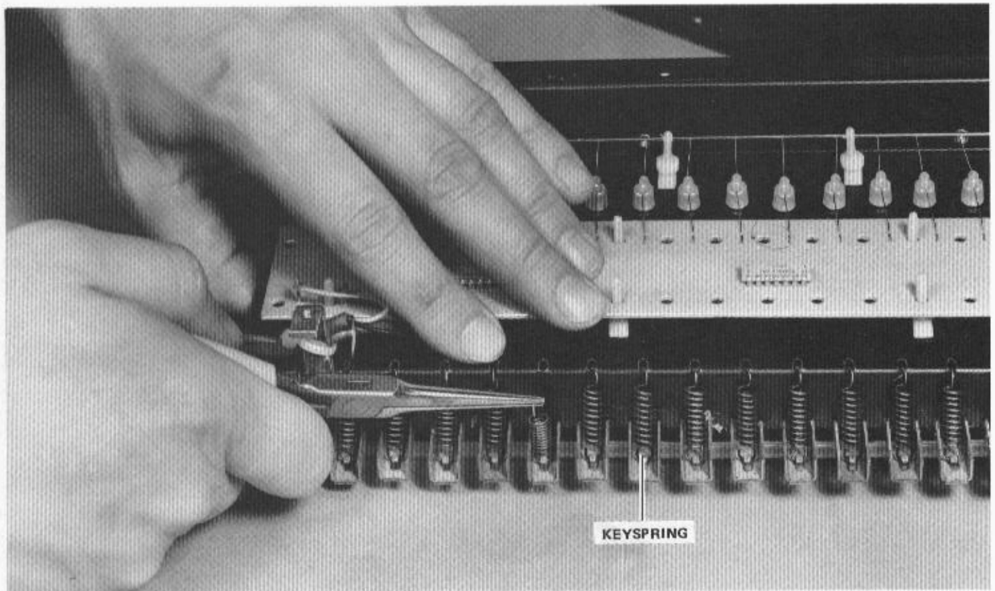
FIGURE 3-10 KEYSRING REPLACEMENT
