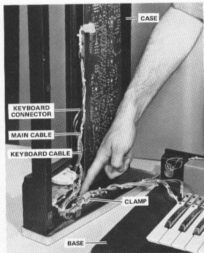
FIGURE 3-3 UNLOCKING CABLE CLAMP
