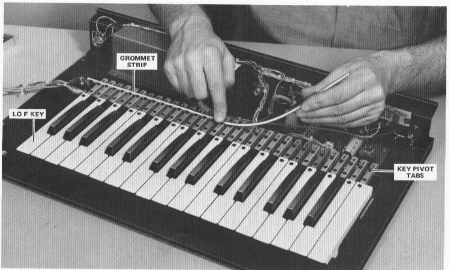
FIGURE 3-5 INSTALLATION OF GROMMET STRIP
